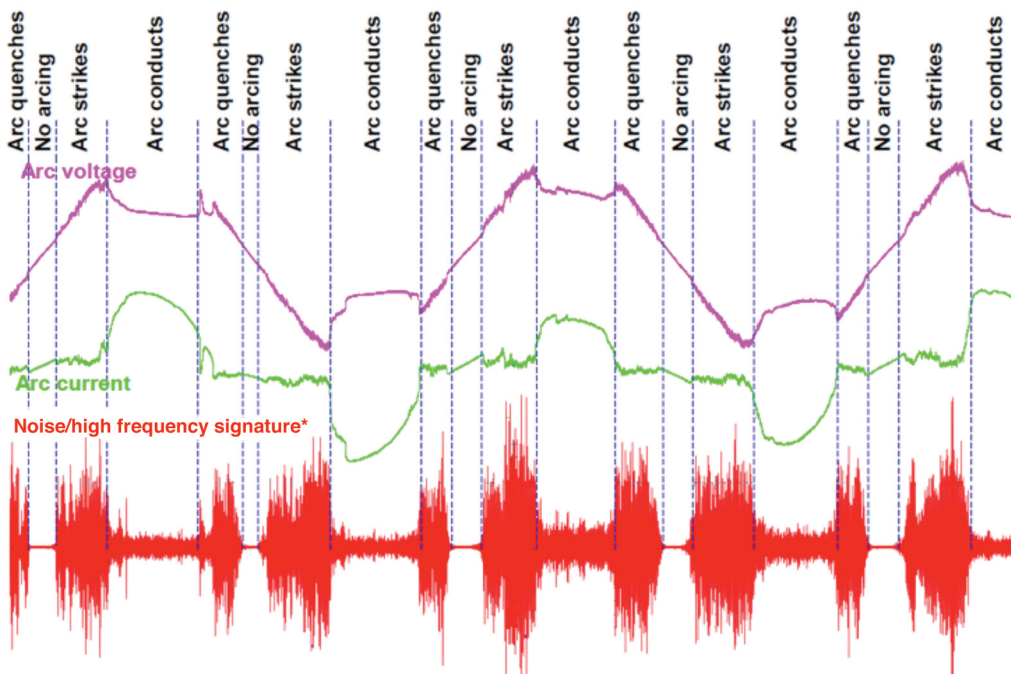
FIGURE 3 – TYPICAL SIGNATURE OF AN ELECTRIC ARC
